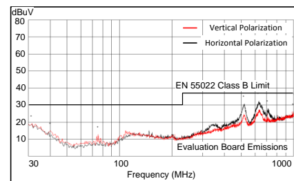
Radiated Emission Graph V_{OUT} = 3.3 \text{ V} , V_{IN} = 24 \text{ V} , F_S = 500 \text{ kHz} , I_{OUT} = 1 \text{ A}
